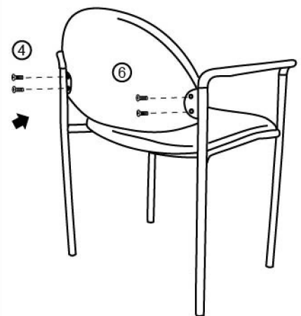
3 Back Joint
